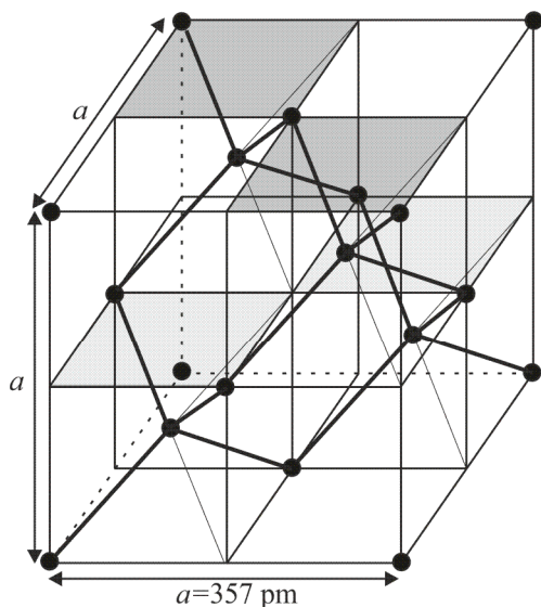
carbone diamant
