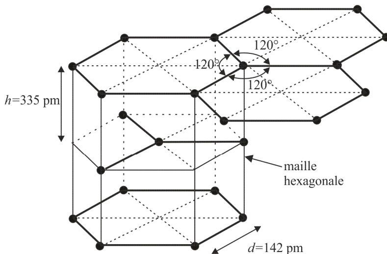
carbone graphite
